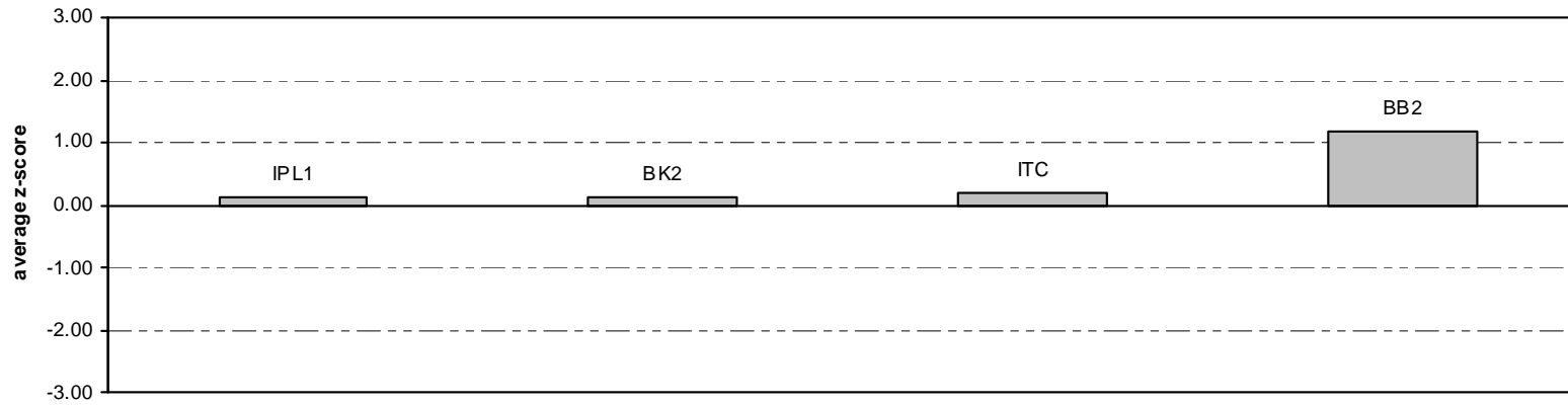
AVGAS - Participant Average Absolute Z-scores
